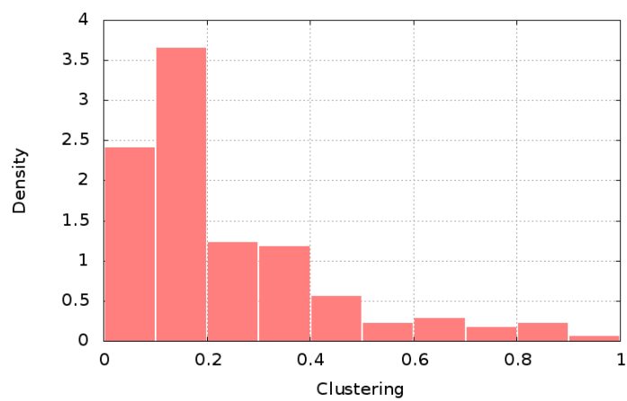
Figure 9: CLUSTERING
